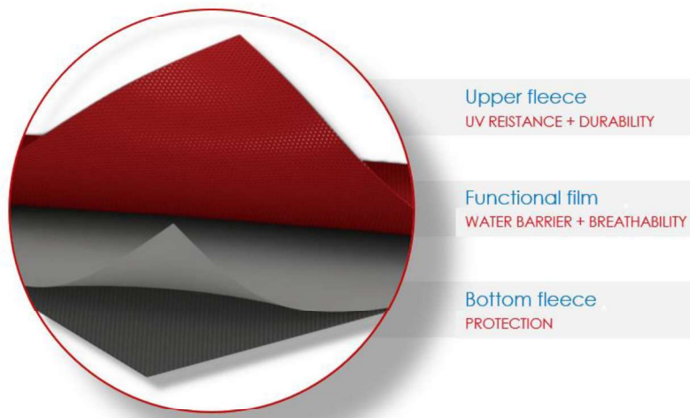
Figure 1 Construction of membrane
